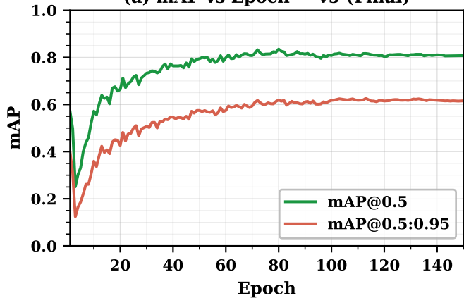
(a) mAP vs Epoch — v5 (Final)
