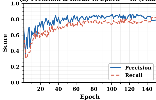
(b) Precision & Recall vs Epoch — v5 (Final)
